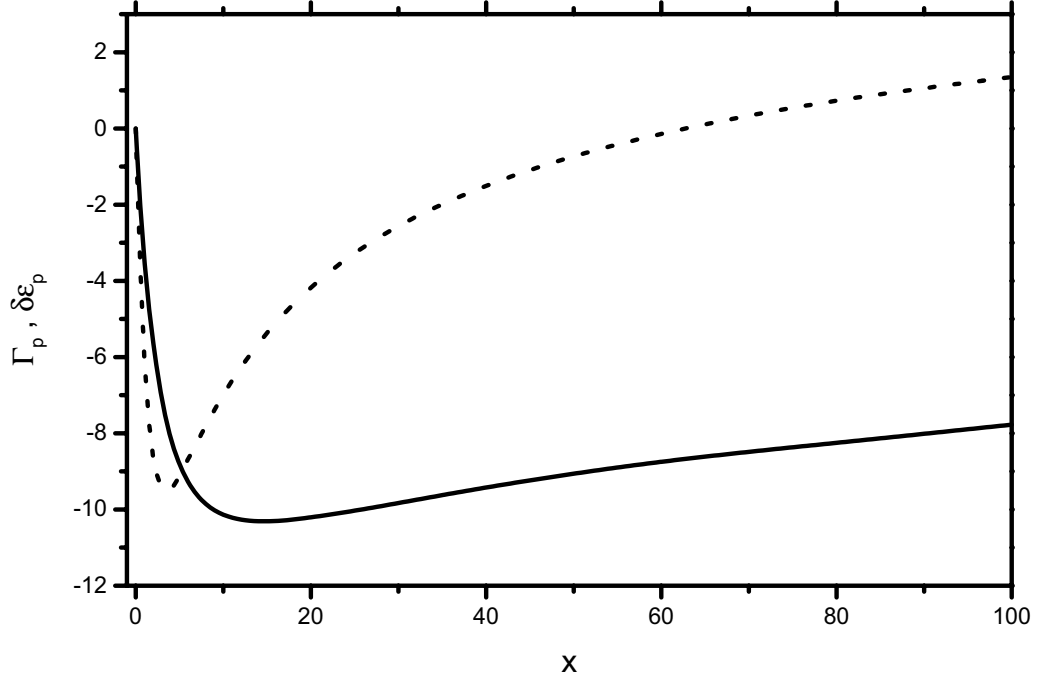
FIGURE 5.3.1. The damping rate \Gamma_p (solid line) and the energy shift \delta\epsilon_p (dashed line) versus x = (\epsilon_p/n_0\tilde{U}) . Both \Gamma_p and \delta\epsilon_p are given in the units of T(n_0a^3)^{1/2} .
